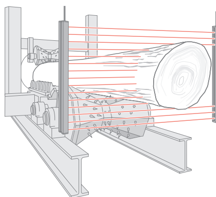
FORESTRY Log measuring
